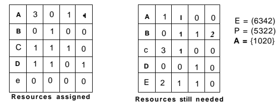
Figure 6-12. The banker's algorithm with multiple resources.
