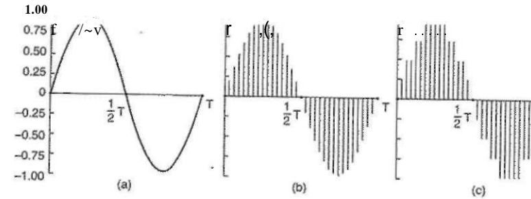
Figure 7-5. (a) A sine wave, (b) Sampling the sine wave, (c) Quantizing the samples to 4 bits.
