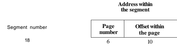
Figure 3-36. A 34-bit MULTICS virtual address.
